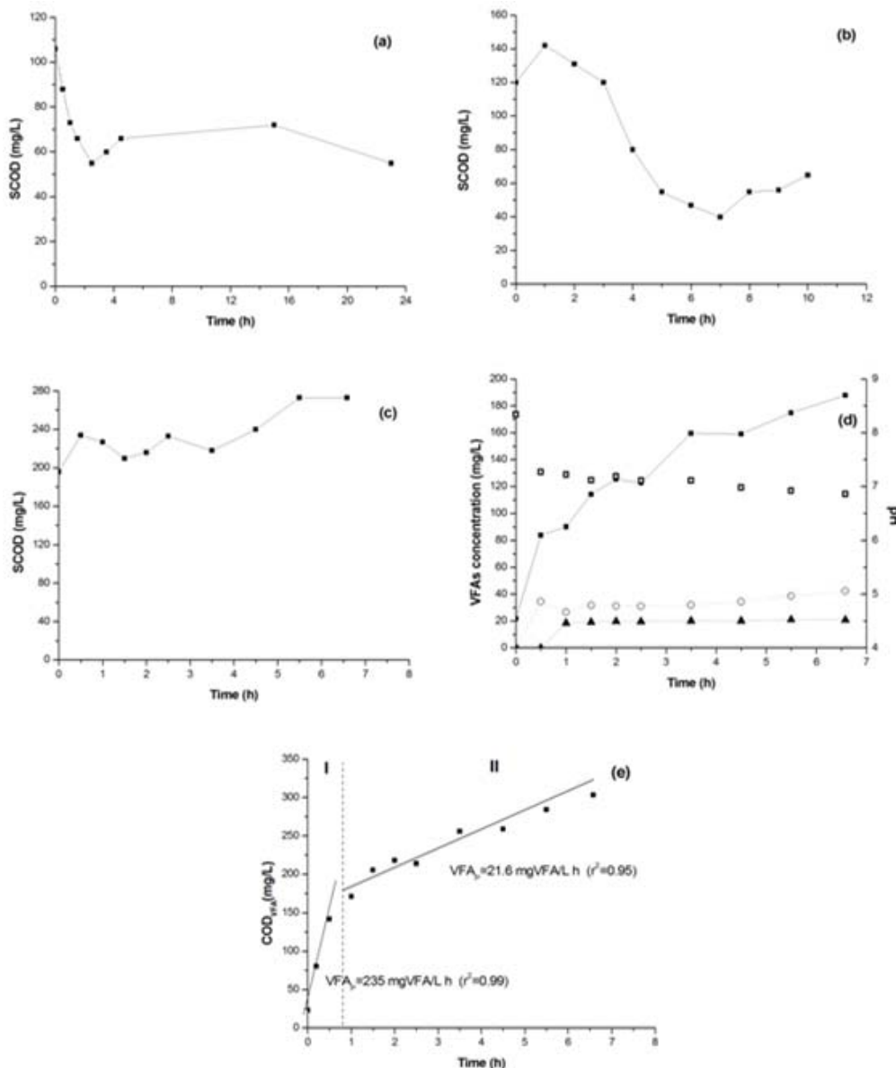
Figure 4. sCOD concentrations during the reaction stage of: (a) phase I; (b) phase II; (c) phase III; (d) VFA concentration variation: (■) Acetic acid (○) Propionic acid and (▲) Butyric acid and (□) pH; (e) VFA-COD equivalent during the reaction stage of phase III.
