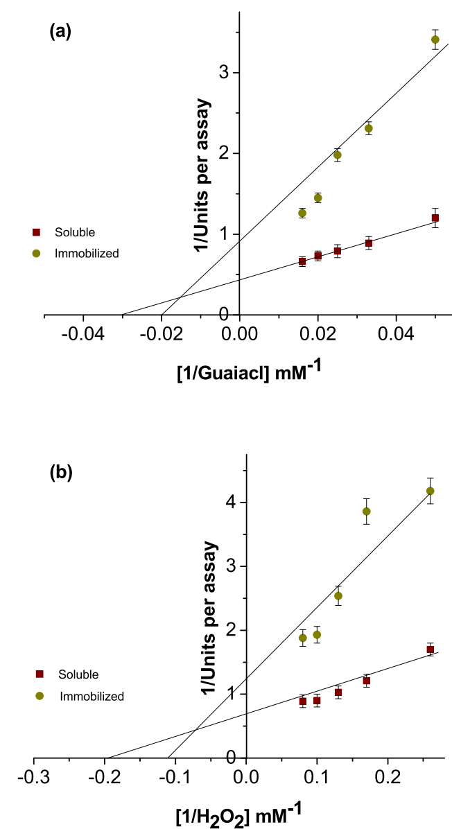
Fig. 7. Lineweaver-Burk plot relating soluble HRP and HRP immobilized on Fe 3 O 4 magnetic nanoparticle reaction velocity to guaiacol (a) and H 2 O 2 (b) concentrations. Each point represents the average of three experiments \pm S.E.
