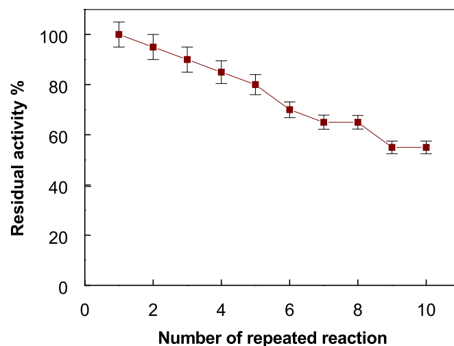
Fig. 5. Reuse of HRP immobilized on \text{Fe}_3\text{O}_4 magnetic nanoparticle. Each point represents the mean of three experiments \pm S.E.
