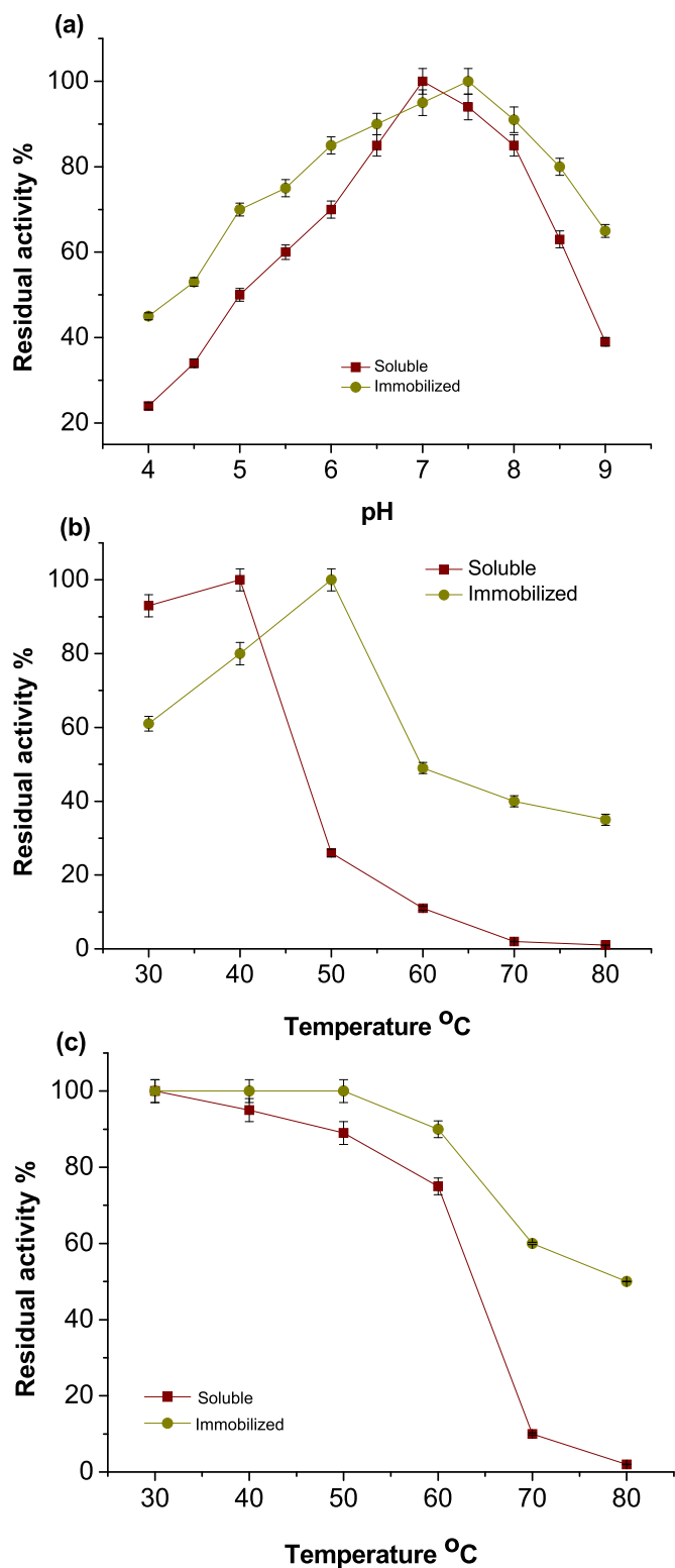
Fig. 6. Optimum pH (a), optimum temperature (b), and thermostability (c) of soluble HRP and HRP immobilized on Fe 3 O 4 magnetic nanoparticle. Each point represents the average of three experiments \pm S.E.
