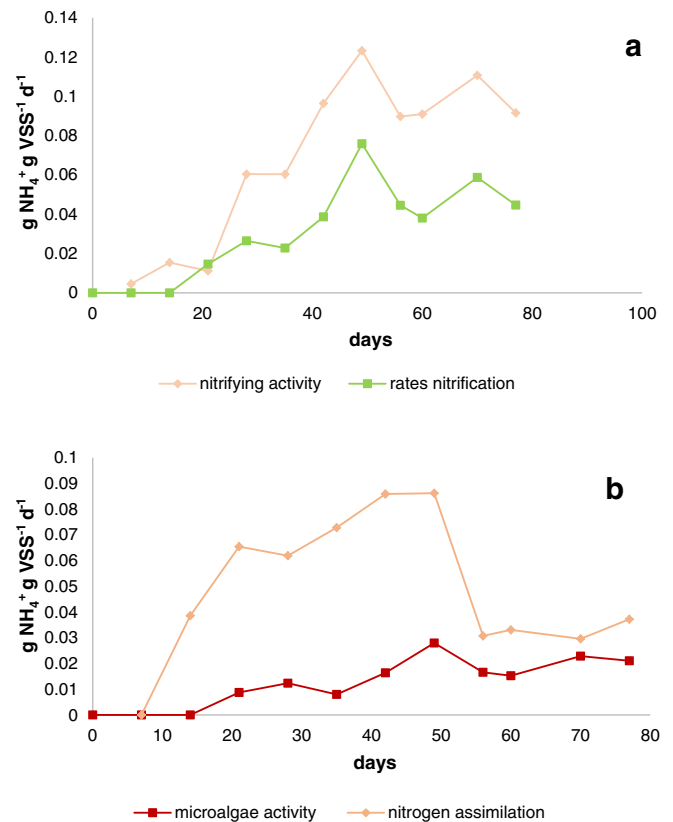
Fig. 4. (a) Evolution of the specific nitrifying activity and rates nitrification. (b) Microalgae activity and nitrogen assimilation in the obtaining of the consortium. The specific activity is determined for the methodology external (off-line), and the rates (in-line parameters) for the balance of nitrogen in the reactor.
