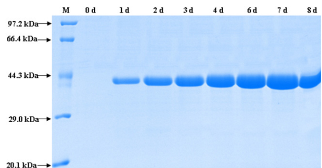
Fig. 2. Time course of AnFaeA expression by P. pastoris GSKZ \alpha FA20 by SDS-PAGE. Lane M: molecular mass standard protein.
