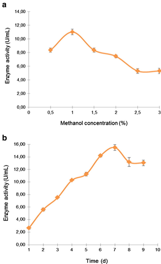
Fig. 1. Effects of induction time and methanol concentration on the expression level of AnFaeA. a: The P. pastoris GSKZ \alpha FA20 was induced in a BMMY medium containing methanol at different final concentrations (0.5–3.0%). b: The P. pastoris GSKZ \alpha FA20 was induced in a BMMY medium by adding methanol of 1.0% at 24-h intervals until 216 h at 28°C.
